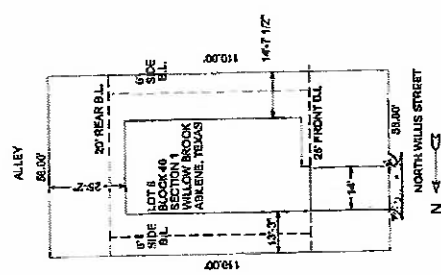
PLOT PLAN 1 in = 20 ft
