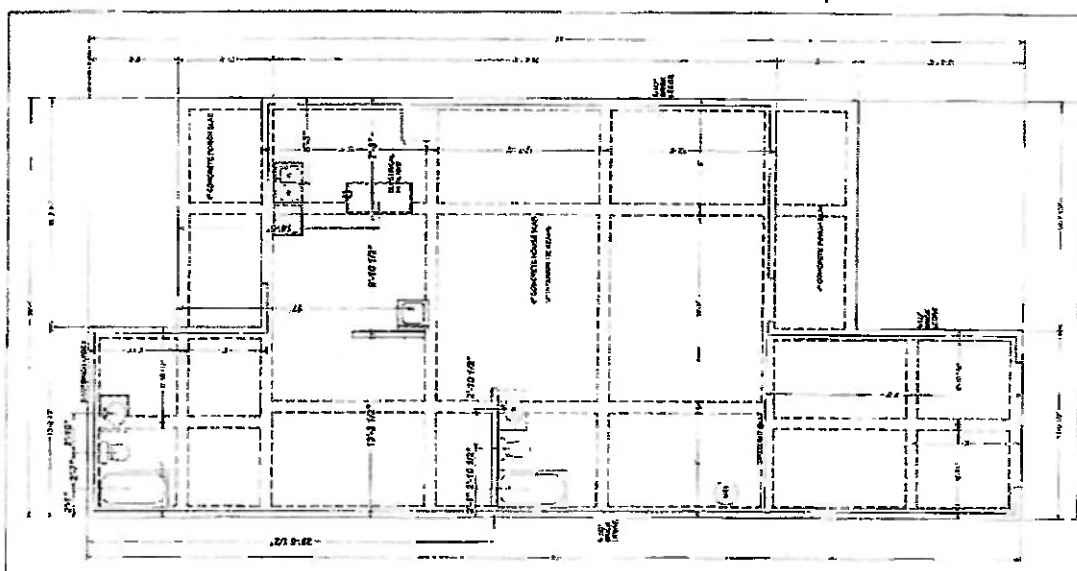
FOUNDATION PLAN 1/8 in = 1 ft
